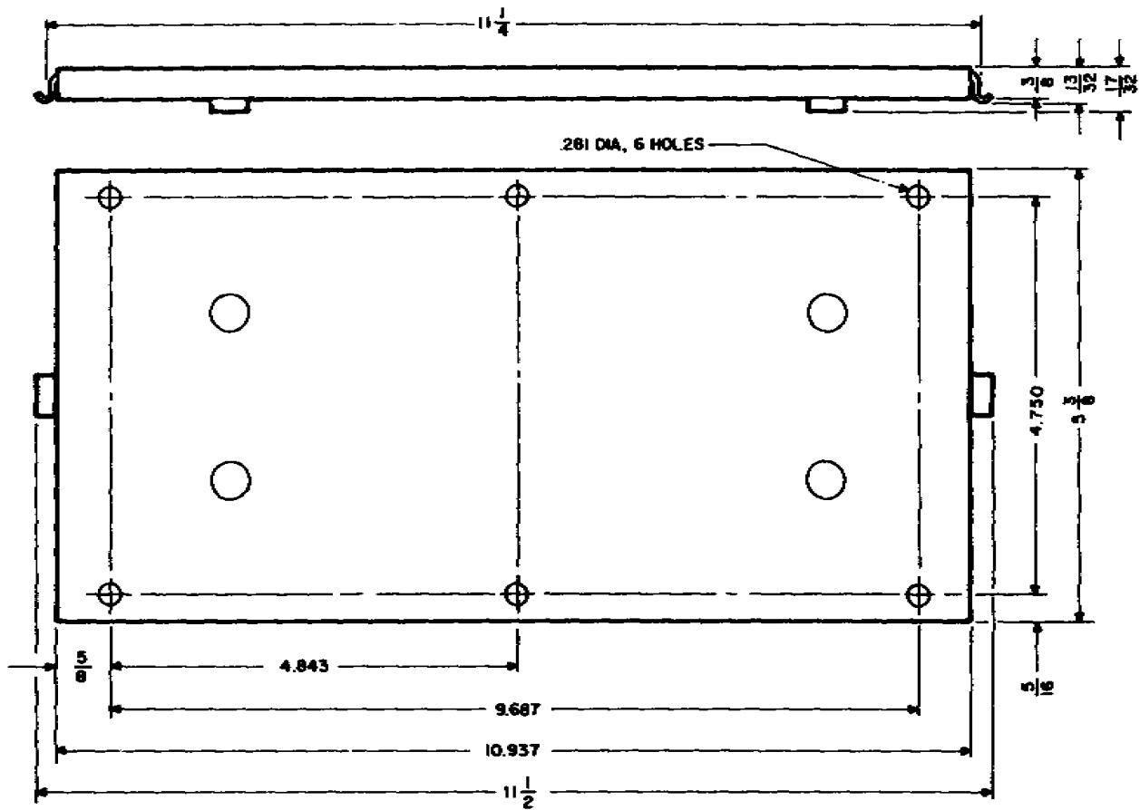
Figure 2-17. Mounting MT-2977/PRC-41. Outline and Mounting Dimensions
